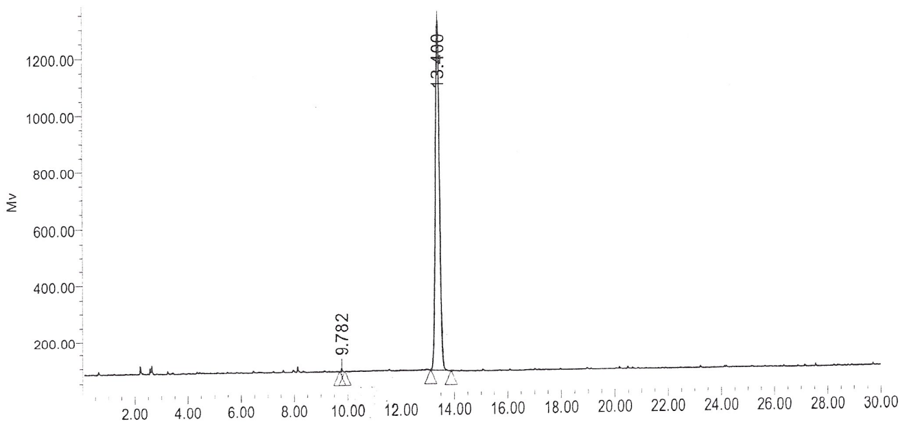
Auto-Scaled Chromatogram
